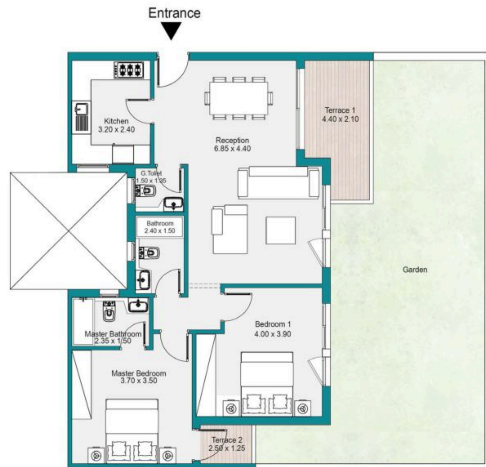
GROUND FLOOR
