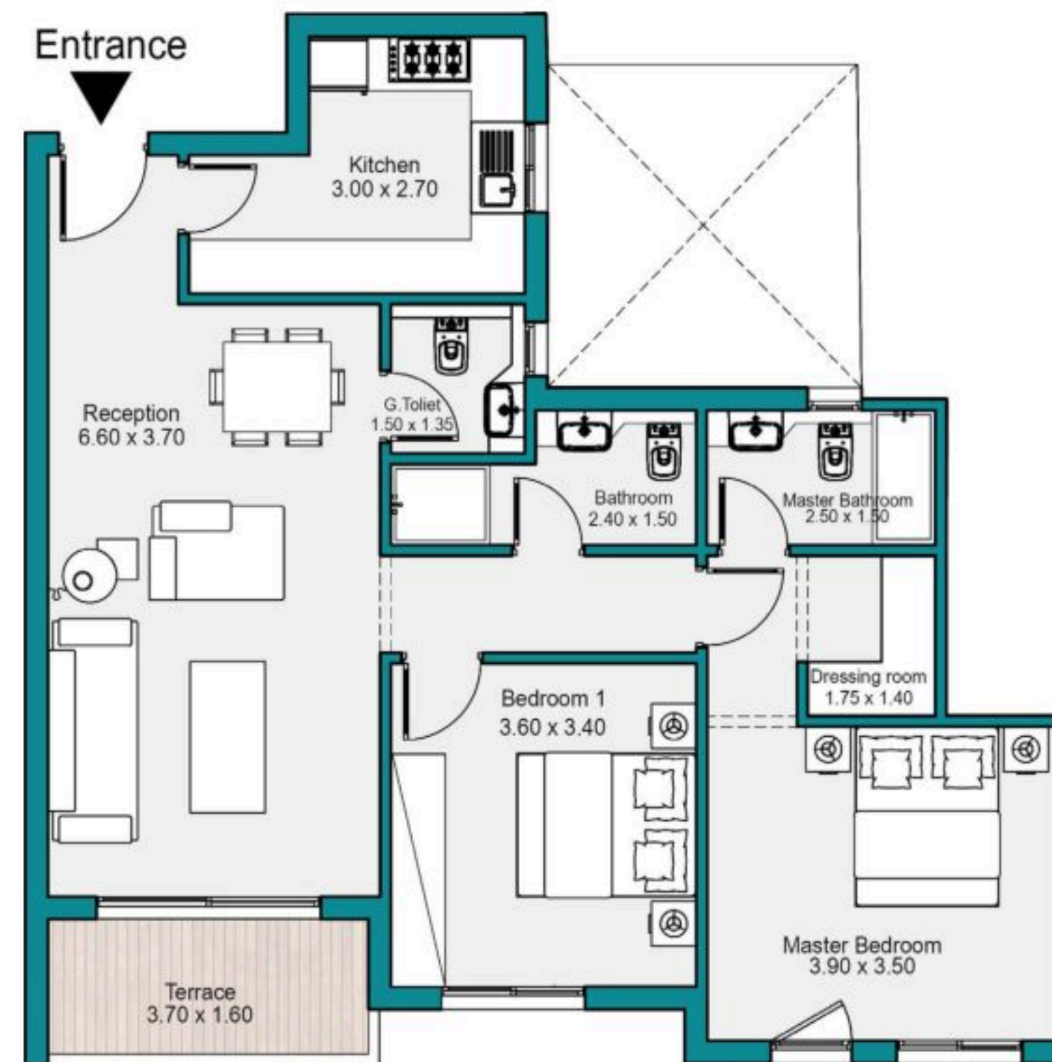
TYPICAL FLOOR
