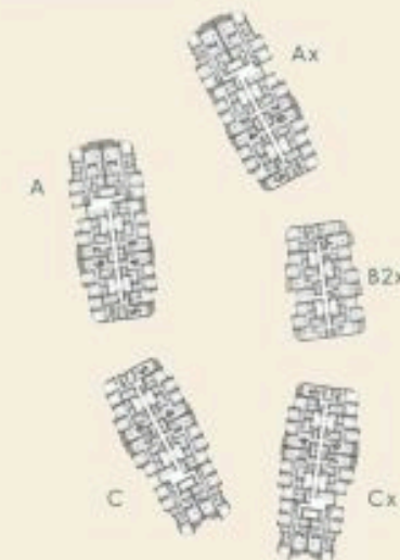
TYPICAL FLOOR
