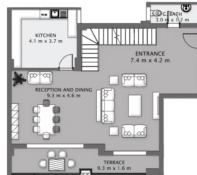
Fourth Floor
