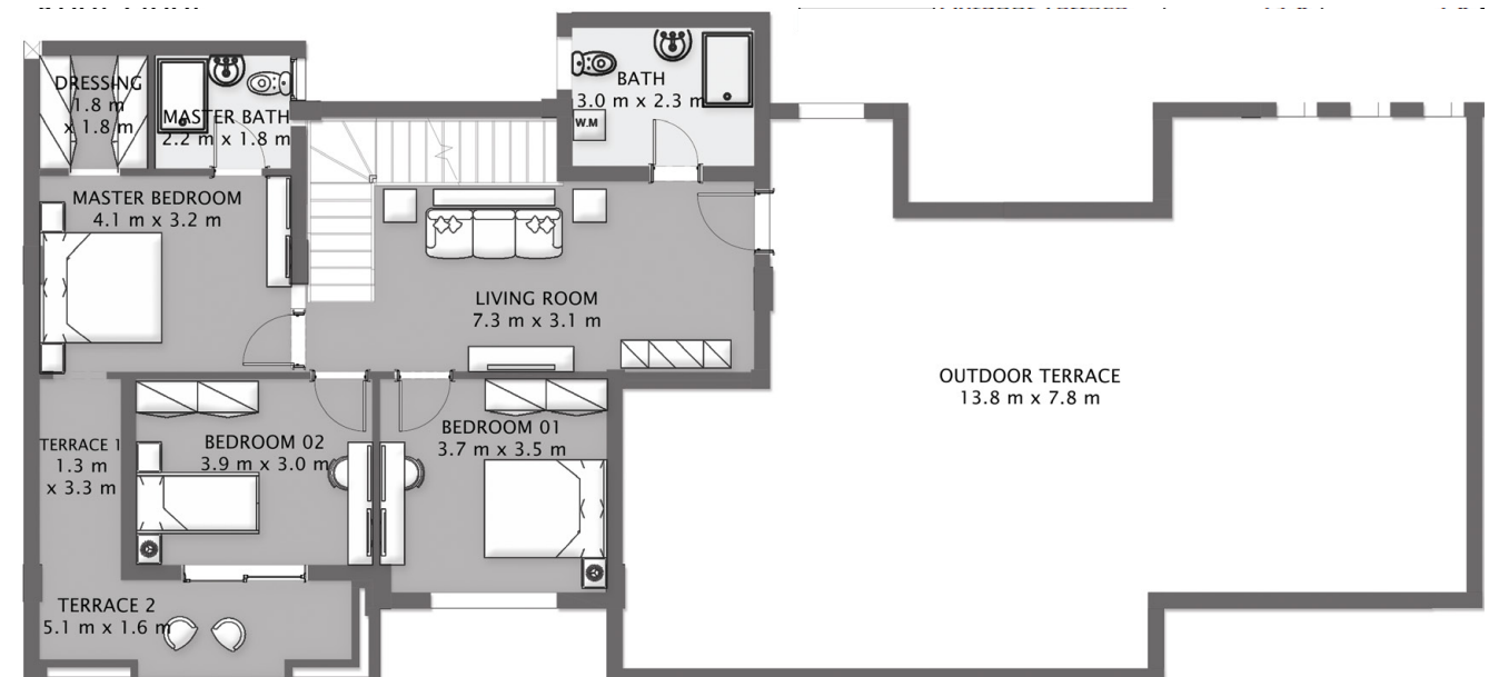
Roof Floor
